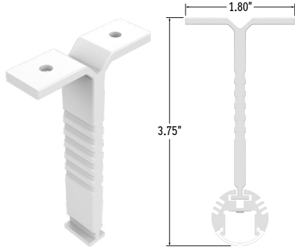
Mounting Bracket (LLED8000-RPM-MB)
