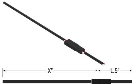
Power Connector Black (20/2 Gauge Wire with Black Jacket) LLED8400-PC (33" Standard) LLED8400-PC-X (X = Specify Length)
