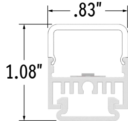
Assembled End View
