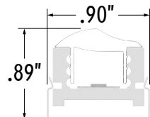
Asymmetric Lens
