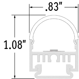
Assembled End View
